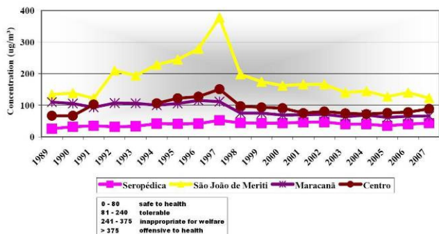
Fig. 2. Annual levels of total particulate matter in the RJMR.
