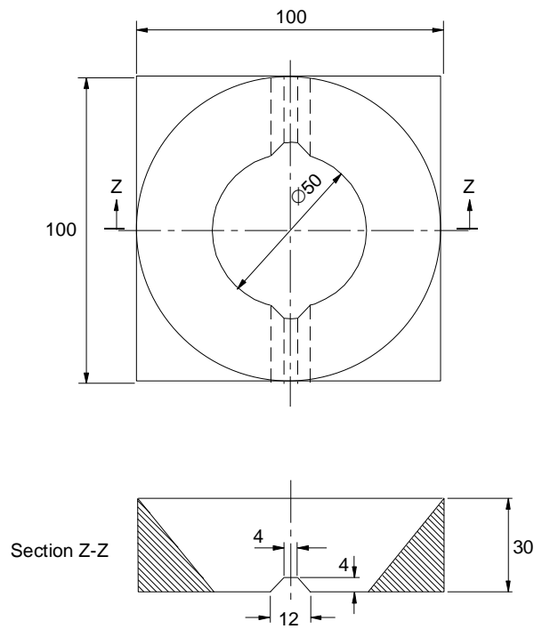
Detail A – Lower part of mask
